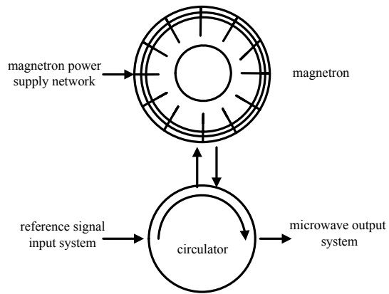
Fig.1 Schematic for inject-locking system 图 1 注入锁频系统框图
