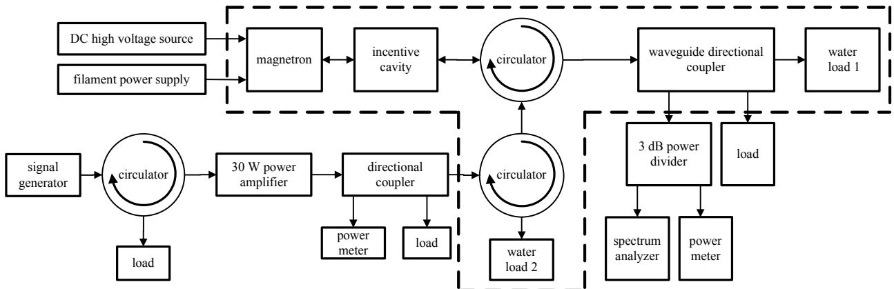
Fig.2 Experimental diagram for magnetron inject-locking system 图 2 磁控管注入锁频系统实验框图
