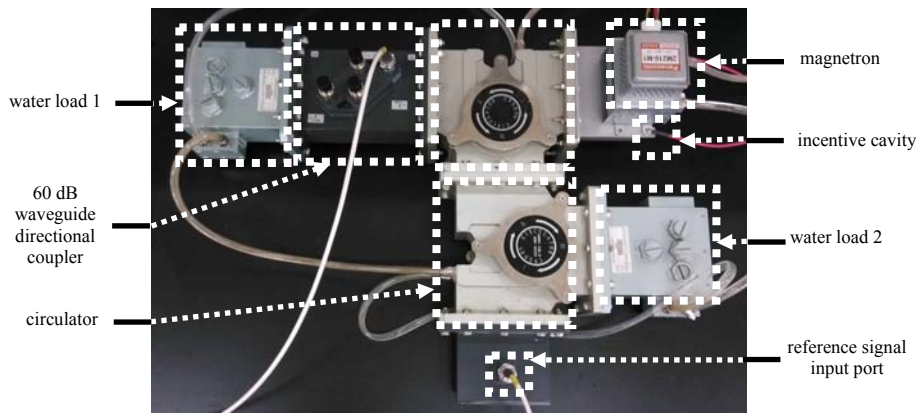
Fig.3 Configuration of inject-locking experimental system 图3 注入锁频实验系统布局图
