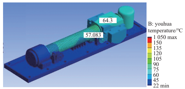
Fig.8 Temperature field distribution after optimization 图 8 优化后温度分布云图
